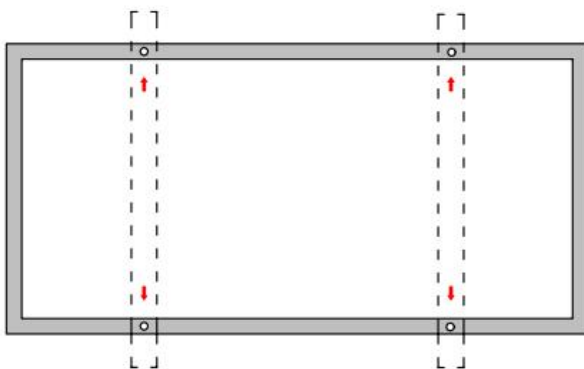
Inner four holes installation method (S-I)
